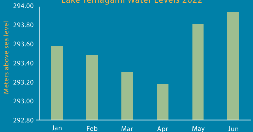
Lake Temagami Water Levels 2022
